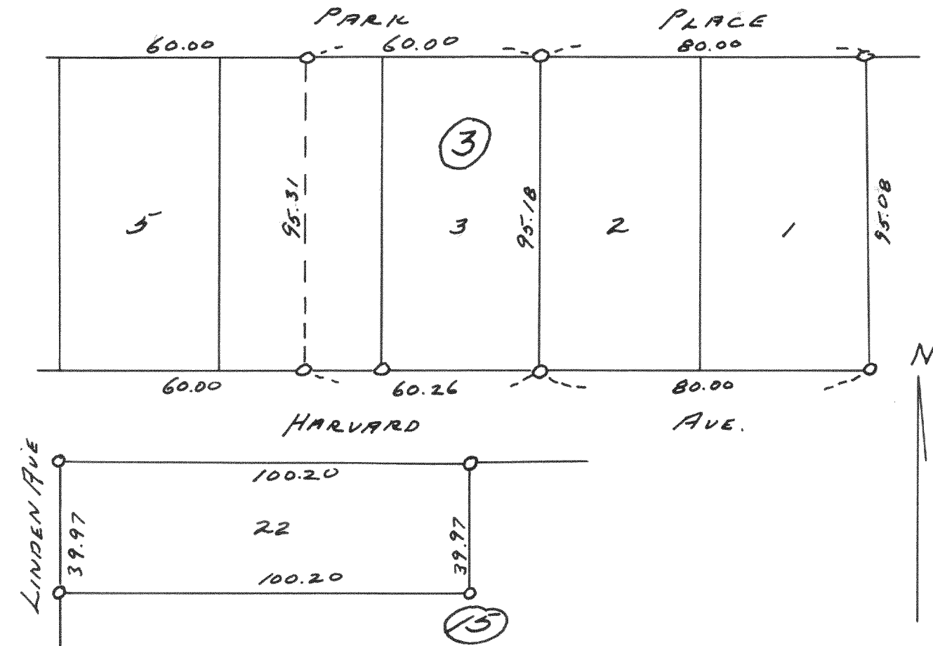
PLAT OF SURVEY OF BLOCK 3 & LOT 22 OF BLOCK 15 GLENWOOD SPRINGS SUBDIVISION VILLAGE OF FONTANA - ON - GENEVA LAKE JULY 1953 LLJ CS
