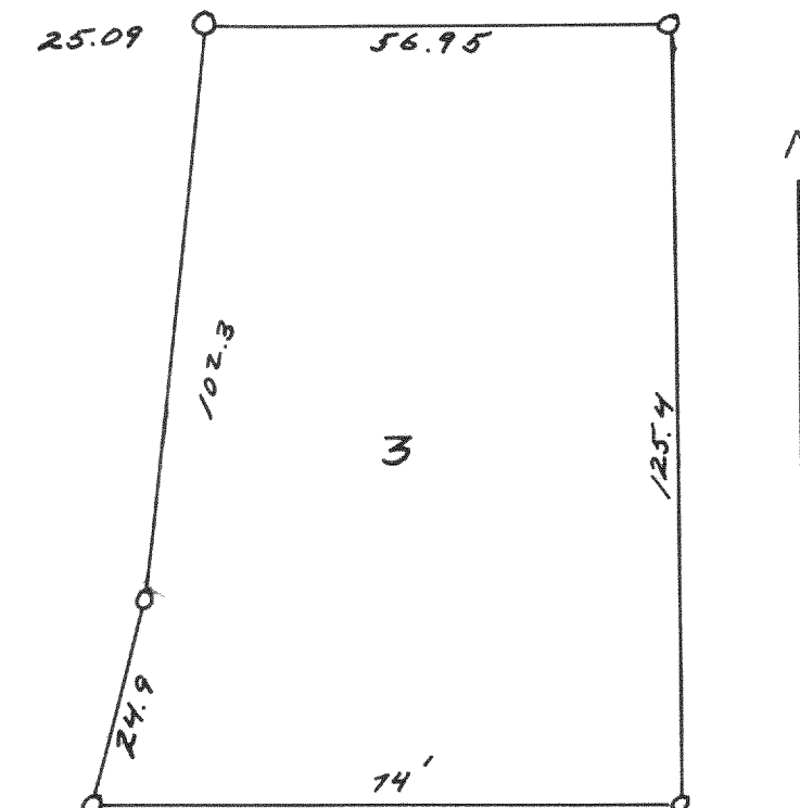
PLAT OF SURVEY OF LOT 3 BLOCK 6 INDIAN HILLS SUB VILLAGE OF FONTANA ON GENEVA LAKE LLJ CS 1953
