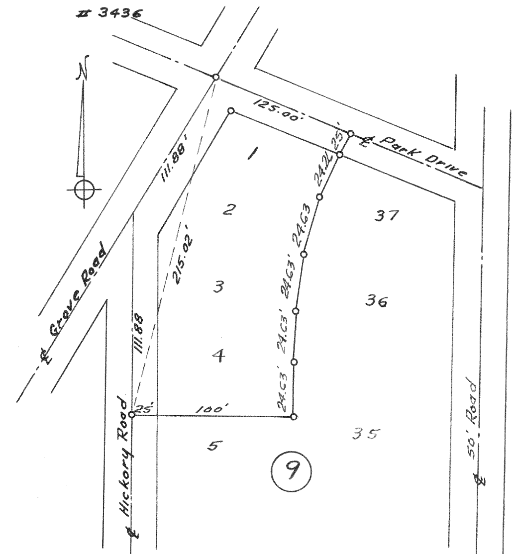
Survey of Lots 1-4 Block 9, Interlaken
