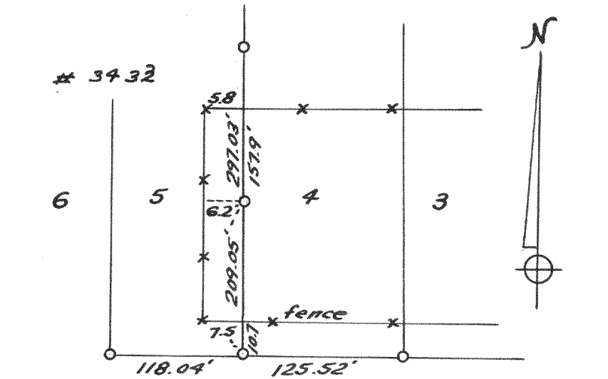
Survey of Lot 5, Hill & Wickstran Subdivision East Delavan, T2N, R16E
