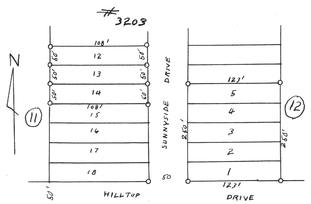
#3203 PLAT OF SURVEY OF LOTS 1-5 BLOCK 12 LOTS 12-14 OF BLOCK 11 MAPLE HILLS T1N R17E WALWORTH COUNTY WISCONSIN NOV. 1956 LLOYD L. JENSEN SURVEYOR
