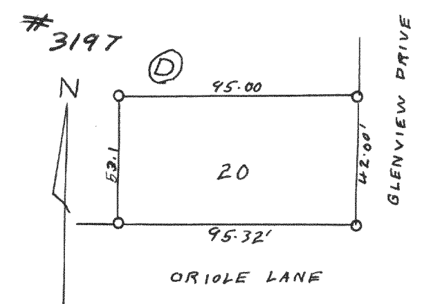
#3197 PLAT OF SURVEY OF LOT 20 BLOCK "D" CISCO BEACH T1N R17E WALWORTH COUNTY WISCONSIN JULY 1956 LLOYD L. JENSEN SURVEYOR
