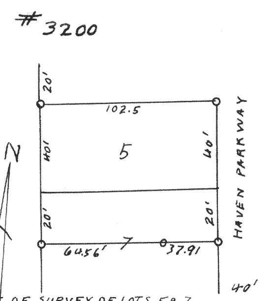
#3200 PLAT OF SURVEY OF LOTS 5 & 7 SHORE HAVEN T1N R17E WALWORTH COUNTY WISCONSIN SEPT. 1956 LLOYD L. JENSEN SURVEYOR
