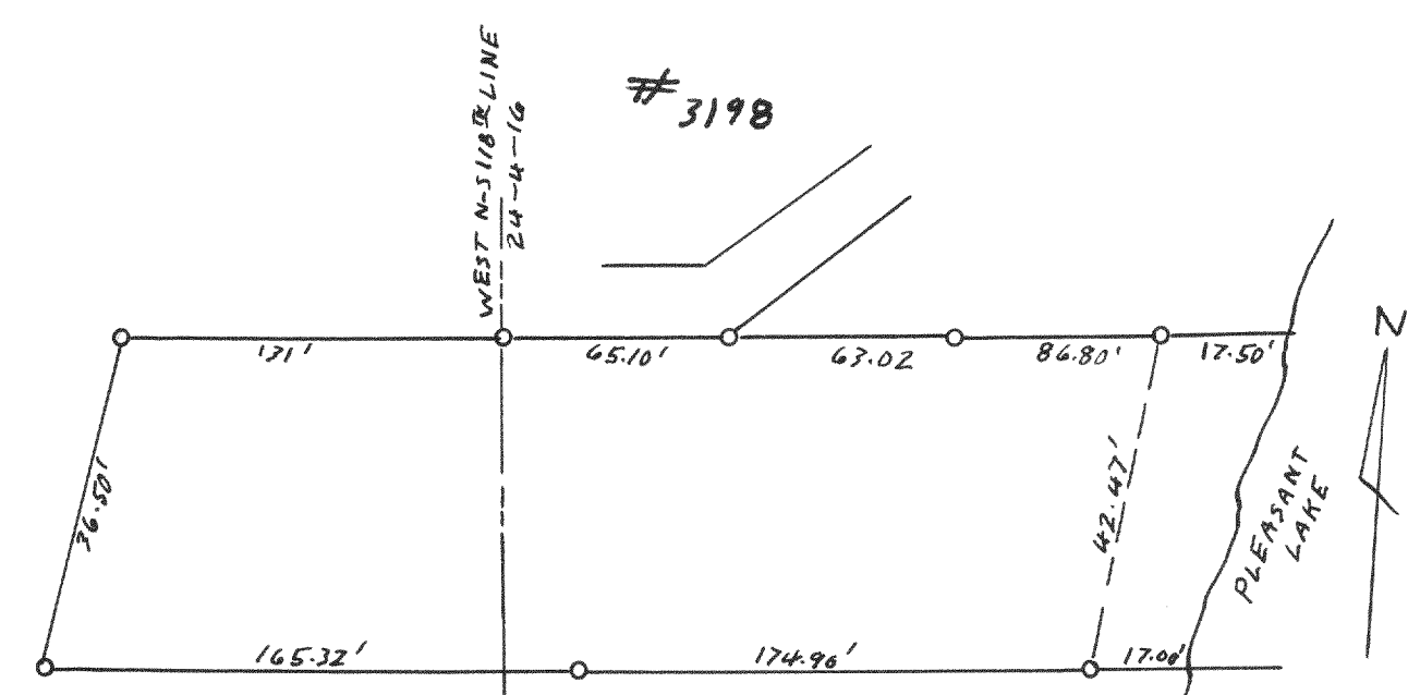
#3198 PLAT OF SURVEY OF PART OF SECTION 24 T4N R16E WALWORTH COUNTY WISCONSIN WALWORTH COUNTY WISCONSIN AUG. 1955 LLOYD L. JENSEN SURVEYOR
