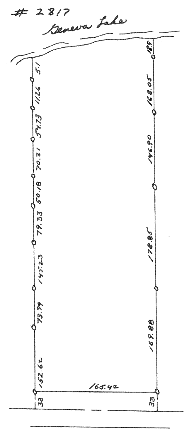
Plat of Survey of West 120 ft. of O.L. 63 Assessor's Plat No. 1 Village of Fontana on Geneva Lake 1953 LLJ CS
