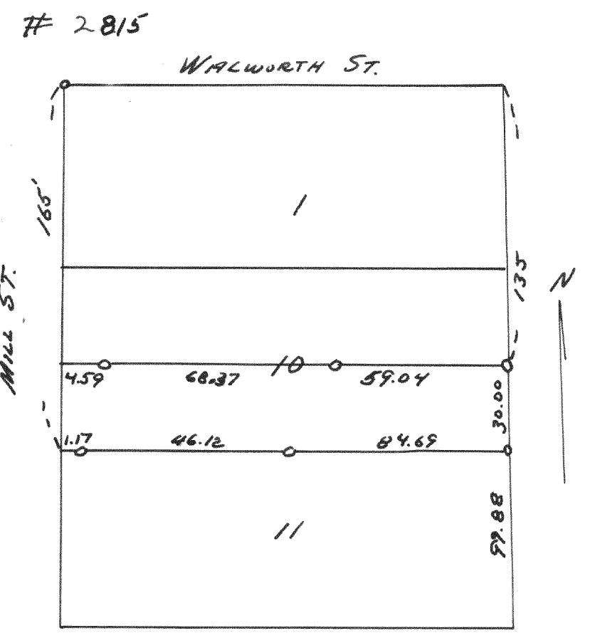
Plat of Survey of Lots 1, 10 & 11 Village of Genoa City, original June 9, 1953 LLJ CS
