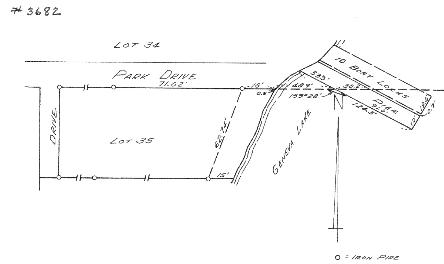
SURVEY OF AREA ADJACENT TO LOT 35 LOCH VISTA CLUB, VILLAGE OF WILLIAMS BAY, WALWORTH COUNTY, WISCONSIN.
