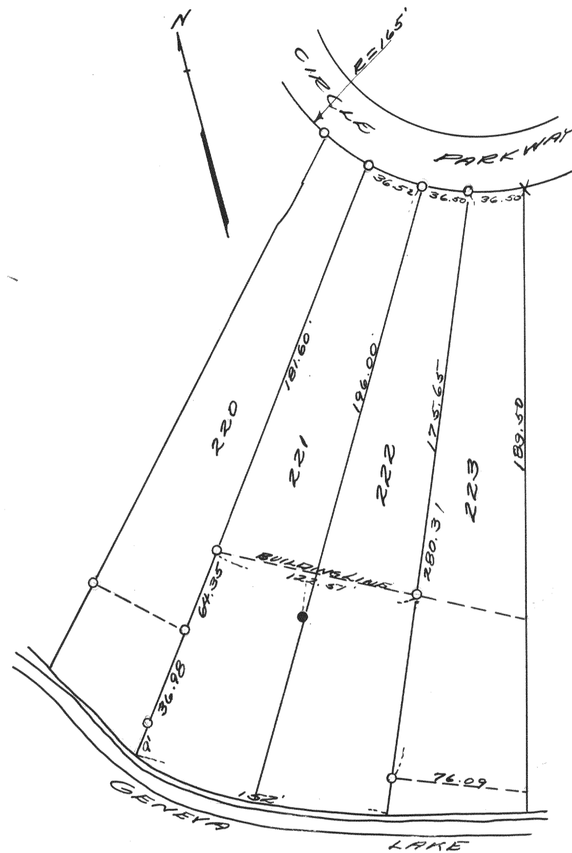
PLAT OF SURVEY OF LOTS 221 & 222 OF THE 3 RD ADDITION TO CEDAR POINT PARK, IN THE VILLAGE OF WIS. BAY, WALWORTH COUNTY, WISCONSIN. Lloyd L. Jensen R.E.J.
