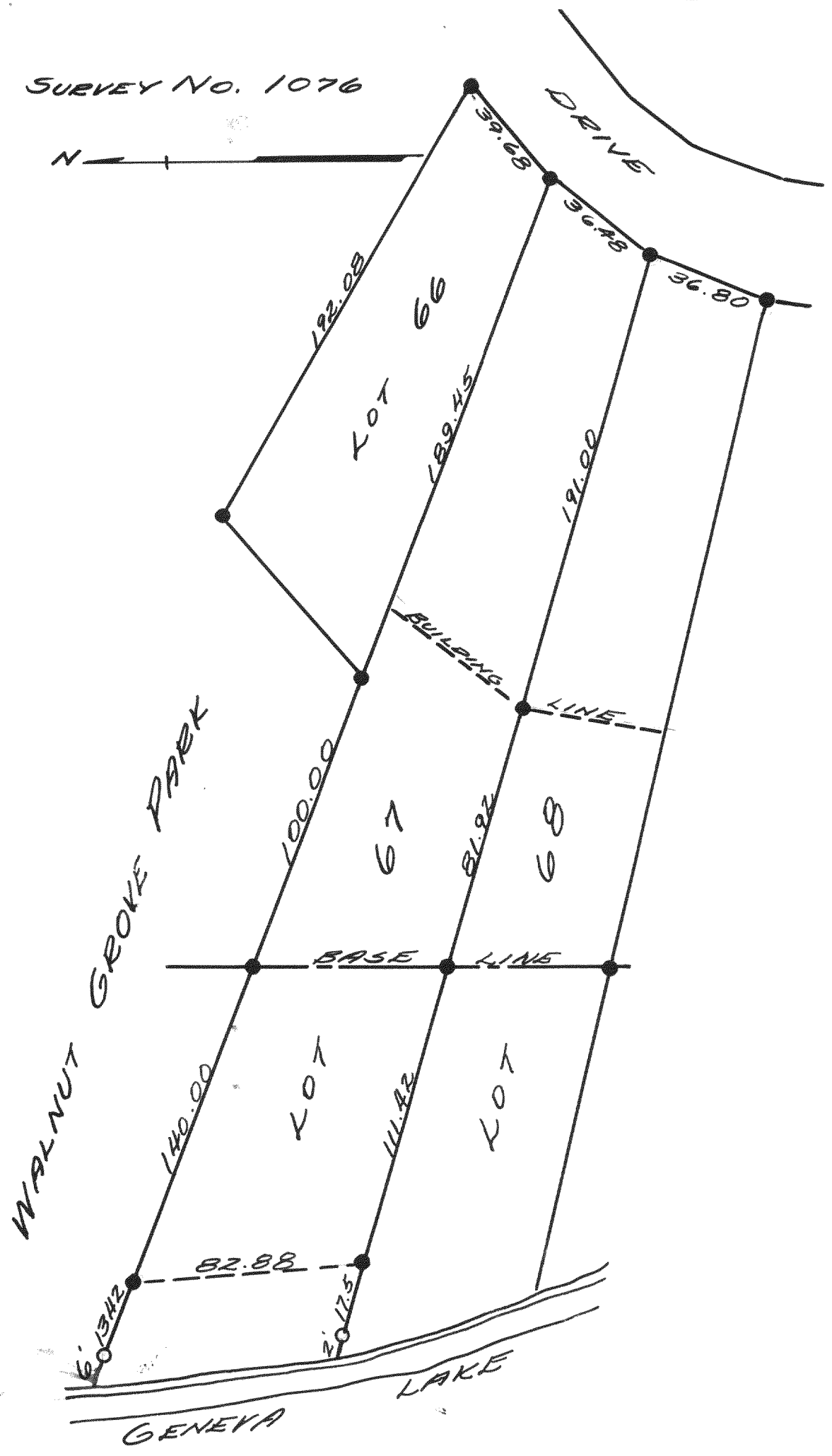
PLAT OF SURVEY OF LOT 67 OF THE FIRST ADD. TO CEDAR POINT IN THE VILLAGE OF WILLIAMS BAY, WALWORTH COUNTY, WISCONSIN.
