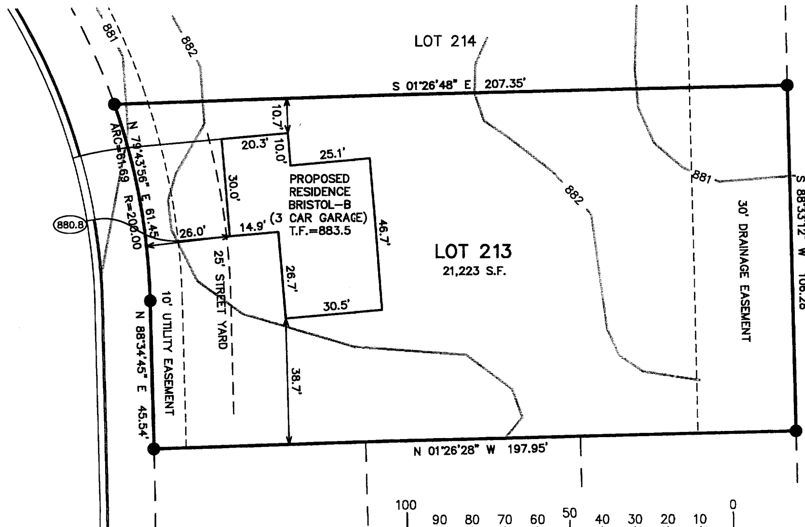
MAP SCALE IN FEET ORIGINAL 1" = 30'
