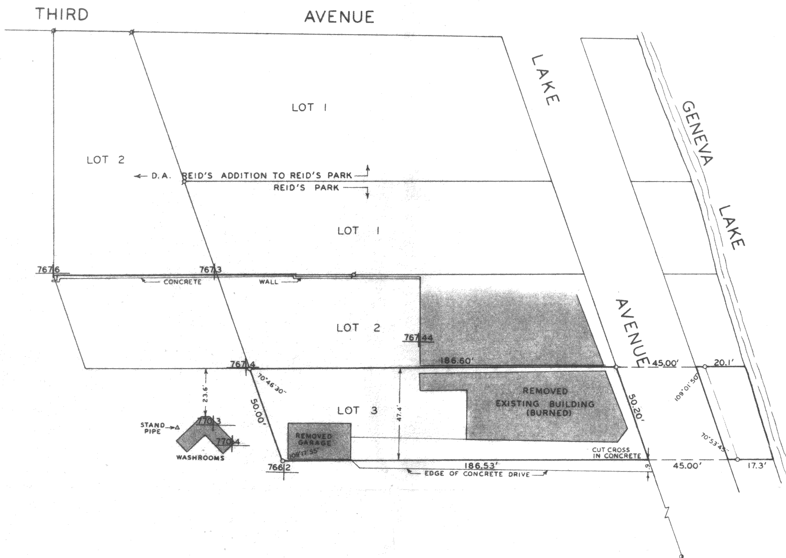
PLAT OF SURVEY OF LOT 3 OF REID'S PARK, VILLAGE OF FONTANA-ON-GENEVA LAKE, WALWORTH COUNTY, WISCONSIN.
