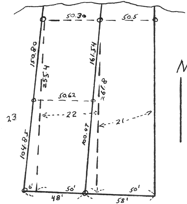
PLAT OF SURVEY OF LOTS 21-23 SHOREWOOD T4N R18E Wakarusa County Wisconsin Nov 1954 LLJ CS
