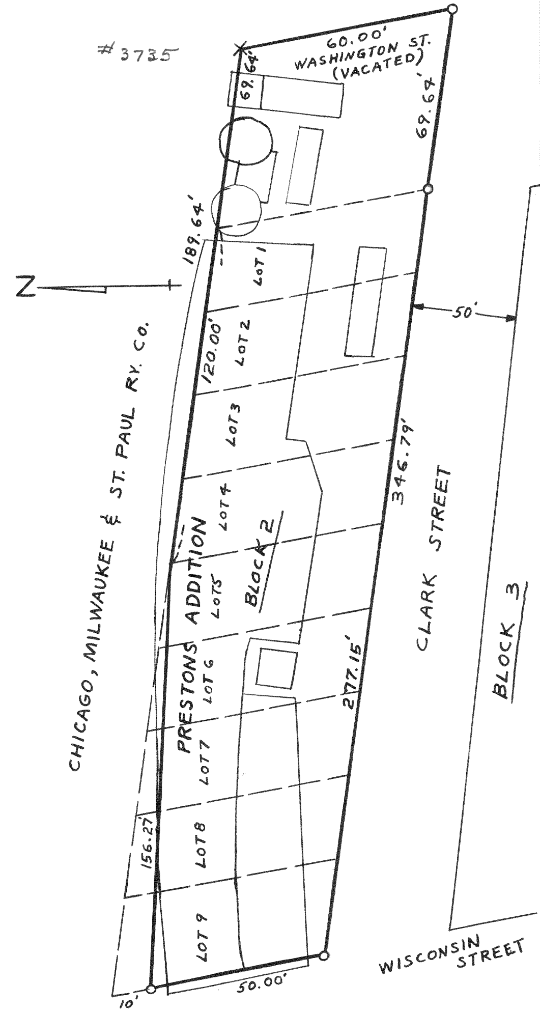
PLAT OF SURVEY OF BLOCK 2, PRESTONS ADDITION AND PART OF WASHINGTON STREET (VACATED), CITY OF ELKHORN, WALWORTH COUNTY, WISCONSIN.
