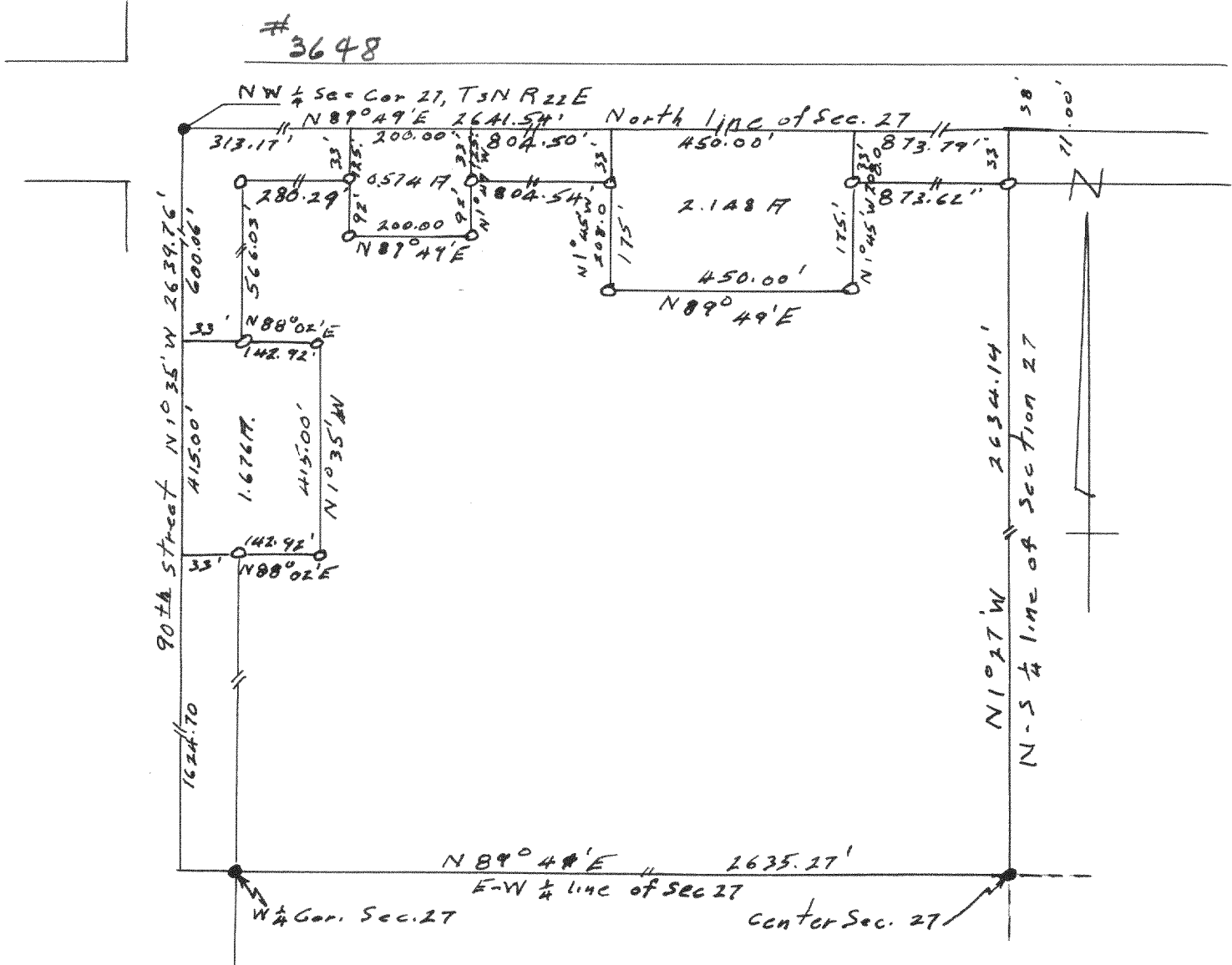
#3648 Plat of survey of the NW 1/4 of section 27, T3N. R22E, Racine County, Wisconsin May 1961 Floyd S. Jensen County Surveyor
