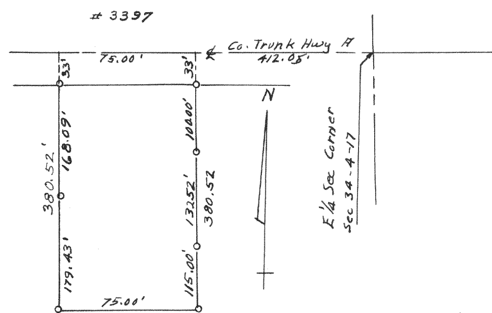
Survey of parcel in SE 1/4 Sec 34-4-17
