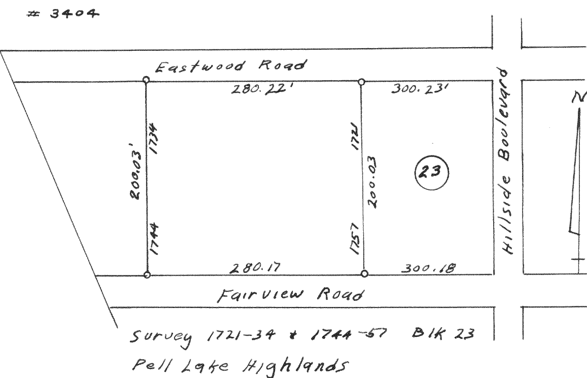
Survey 1721-34 &amp; 1744-57 B1K 23 Pell Lake Highlands
