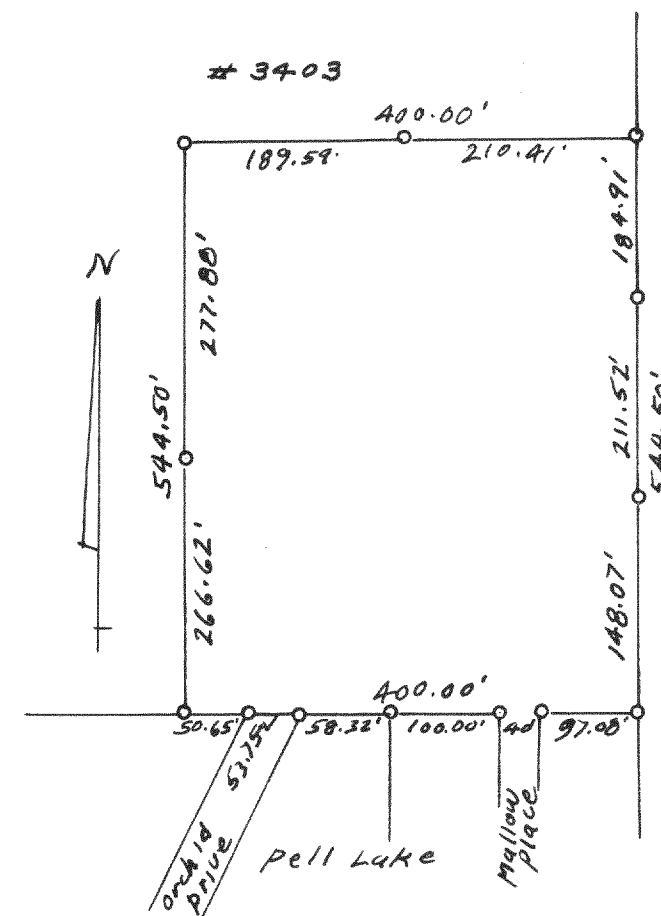
Survey in SW 1/4 SE 1/4 of Section 10, T1N, R18E
