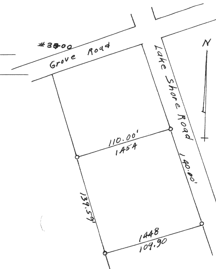
Survey of Lots 1448-54 Pell Lake
