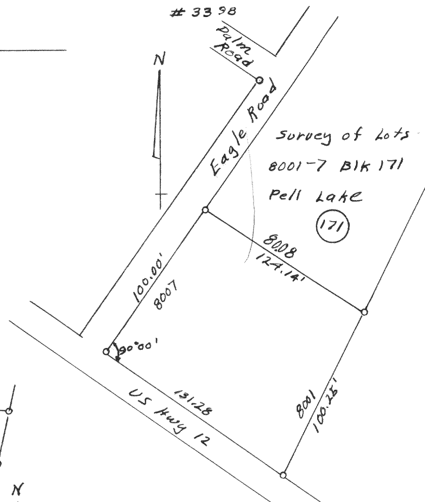
Survey of parcel in SE 1/4 Sec 34-4-17
