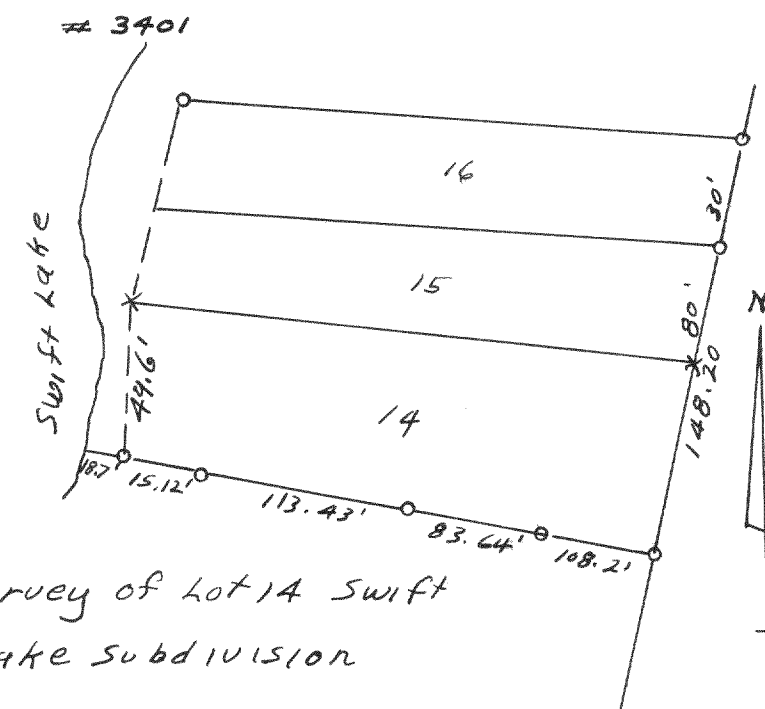
Survey of parcel in SE 1/4 Sec 34-4-17
