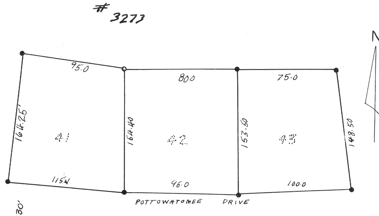
PLAT OF SURVEY OF LOT 41 AND 43 UNIT 2 COUNTRY CLUB ESTATES VILLAGE OF FONTANA ON GENEVA LAKE WALWORTH COUNTY WISCONSIN JULY 1956 LLOYD L. JENSEN SURVEYOR
