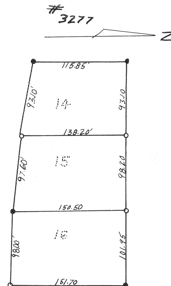
PLAT OF SURVEY OF LOT 14-16 UNIT 2 COUNTRY CLUB ESTATES VILLAGE OF FONTANA ON GENEVA LAKE WALWORTH COUNTY WISCONSIN APRIL 1956 LLOYD L. JENSEN SURVEYOR
