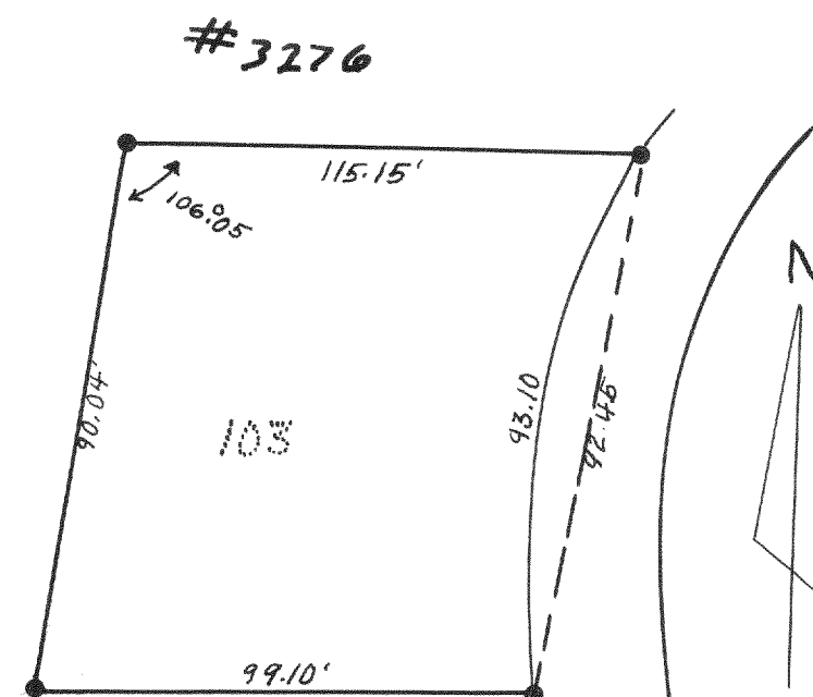
PLAT OF SURVEY OF LOT 103 UNIT 2 COUNTRY CLUB ESTATES VILLAGE OF FONTANA ON GENEVA LAKE WALWORTH COUNTY WISCONSIN JULY 1956 LLOYD L. JENSEN SURVEYOR
