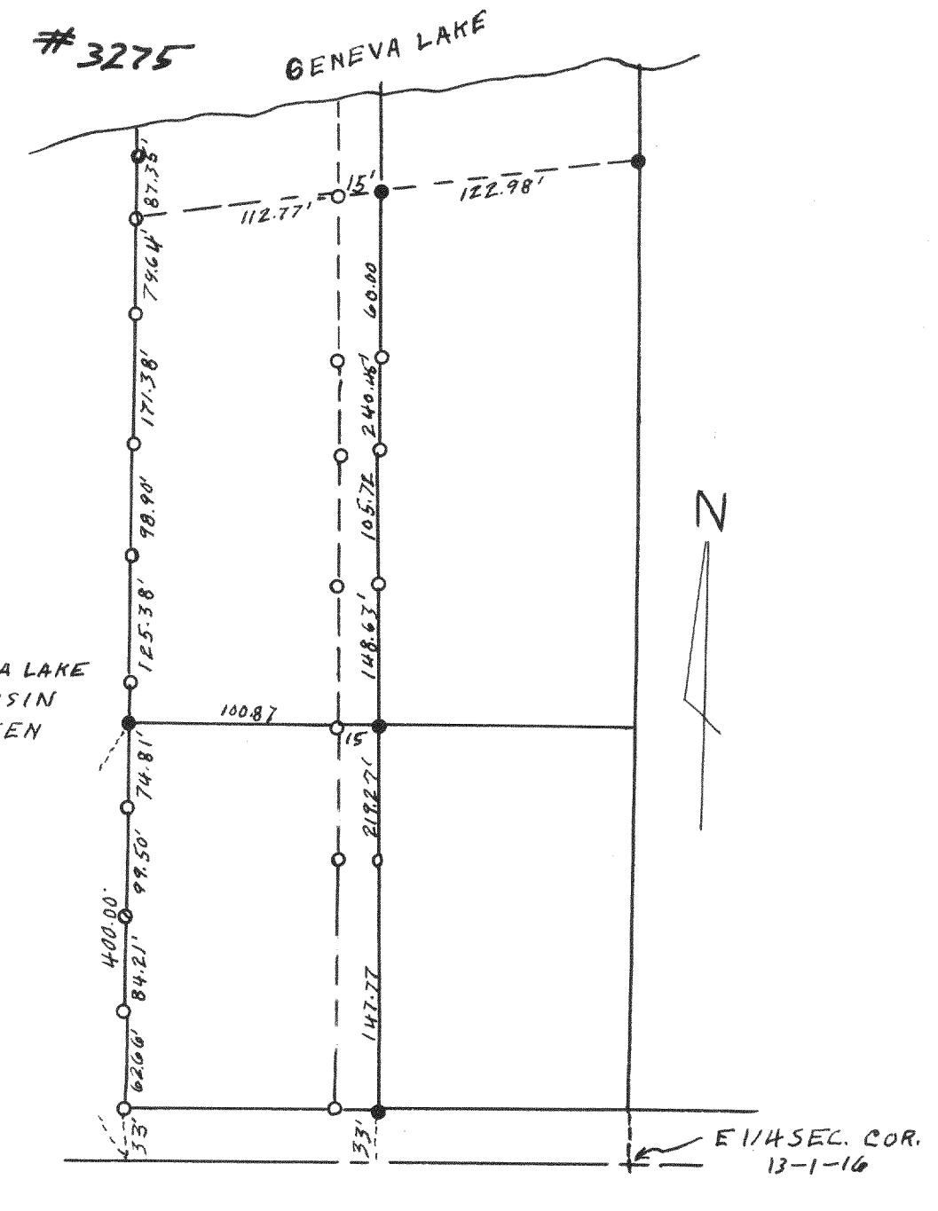
PLAT OF SURVEY OF LAND IN SECTION 13 TIN RICE WALWORTH COUNTY WISCONSIN FEB 1957 LLOYD L. JENSEN SURVEYOR
