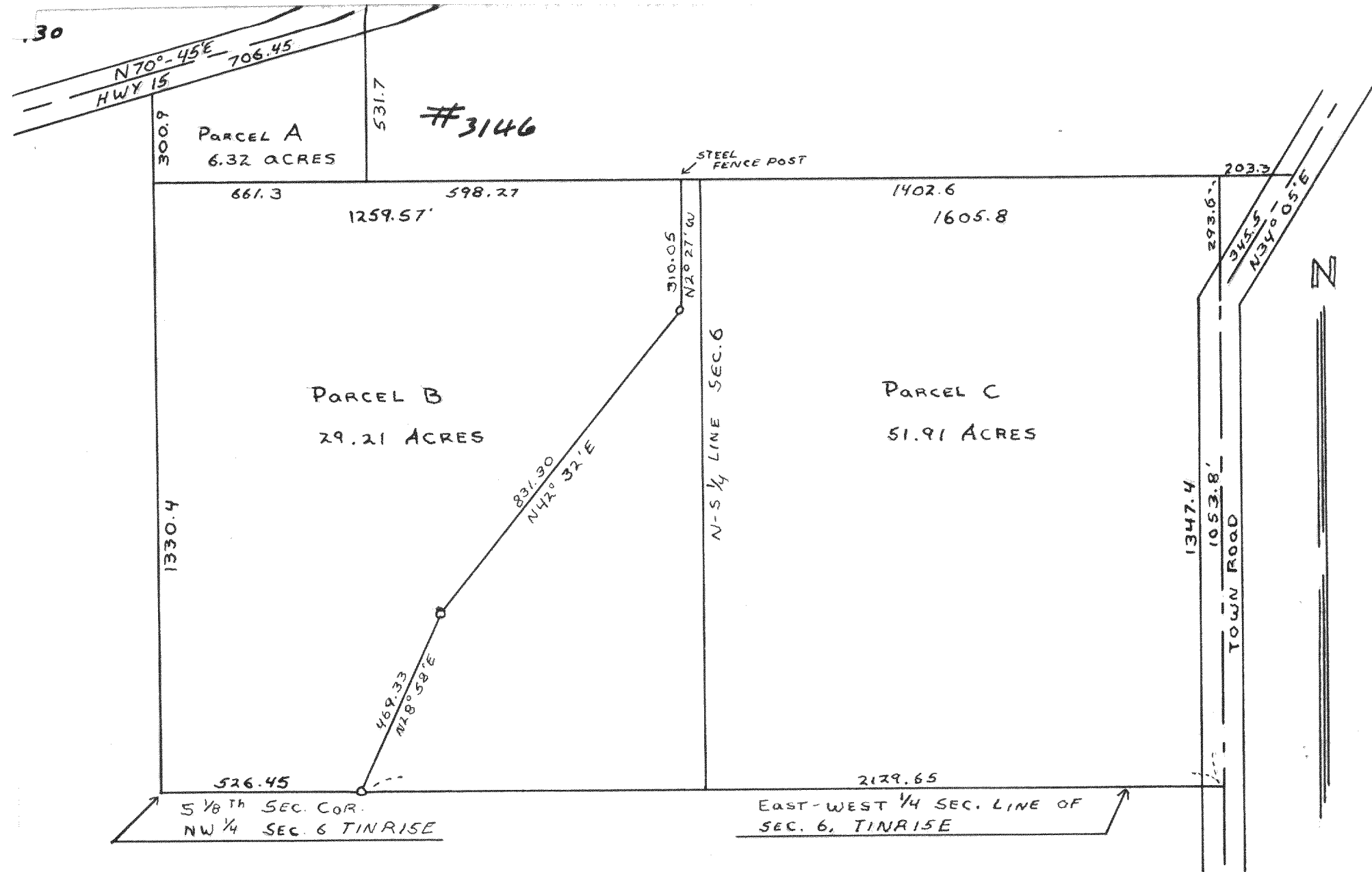
PLAT OF SURVEY OF PARCEL OF LAND IN SEC. 6 T1N R1E WALWORTH COUNTY, WISCONSIN LLOYD L. JENSEN SEPT. 1956 SURVEYOR
