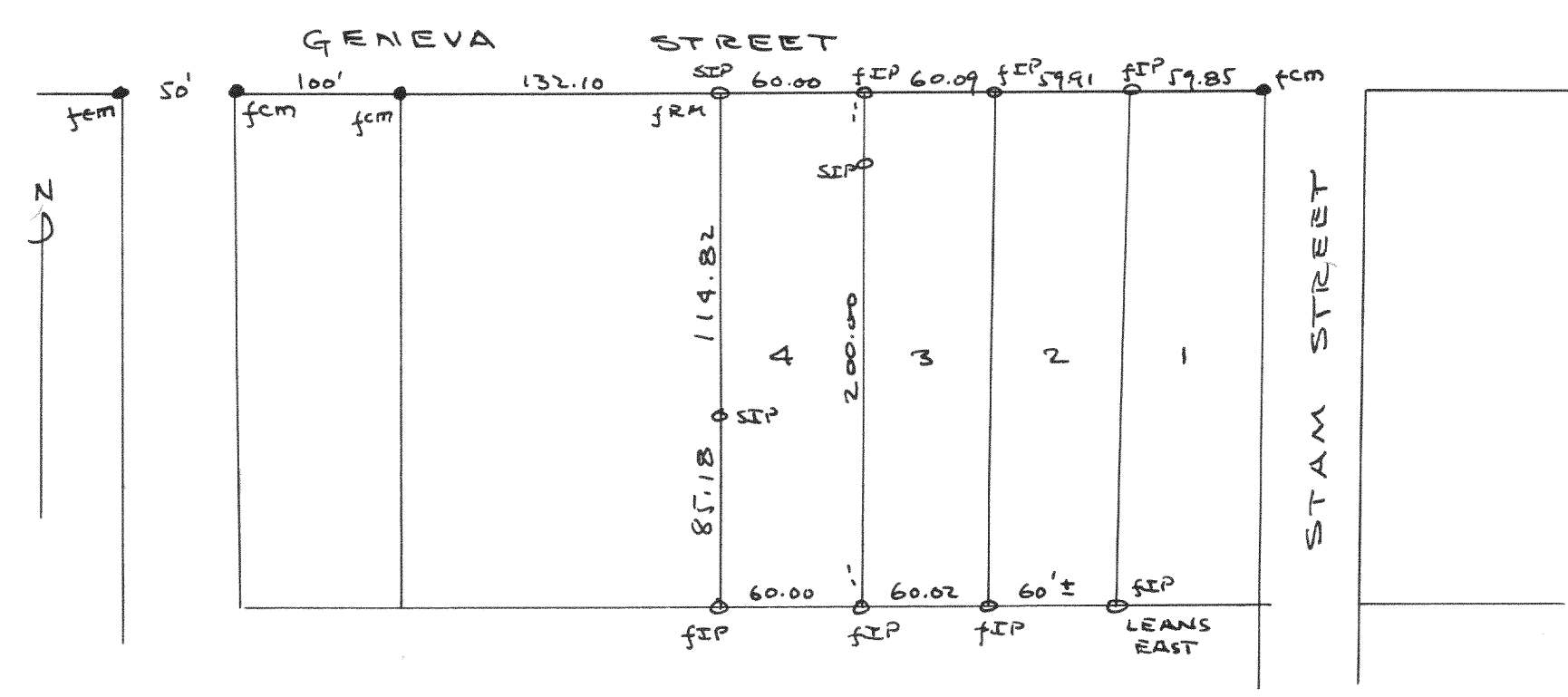
Plat of survey of lot 4, Wm. Pearsons Subdivision, Village of Williams Bay, Section 1, T1N R16E, Walworth County, Wisconsin July 10, 1951 Lloyd L. Jensen JCB County Surveyor
