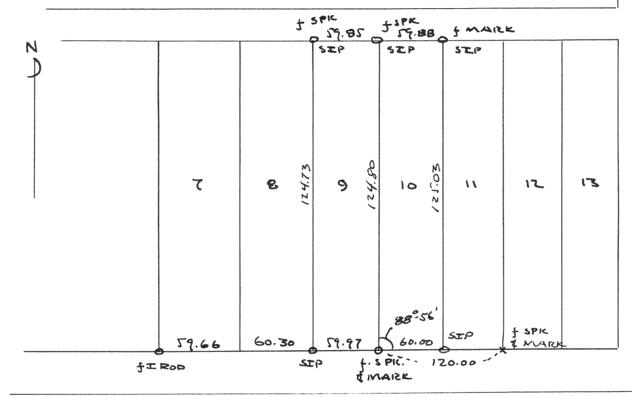
Plat of survey of lots 9 & 10, Lackey Bros. Subdivision, Village of Williams Bay, Section 1, T1N R16E, Walworth County, Wisconsin July 20, 1951 Lloyd L. Jensen JCB County Surveyor
