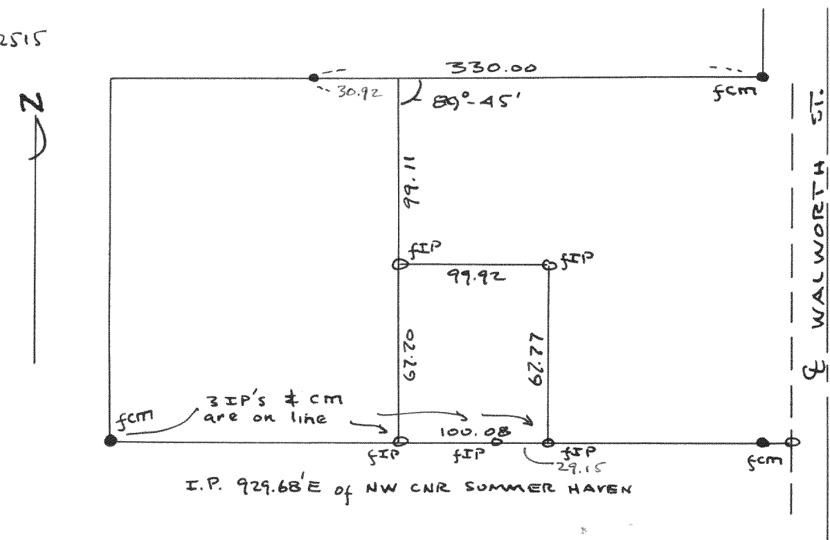
Plat of survey of a parcel of land out of Hatch Estate located in SE 1/4 of Section 1, T1N R16E, Village of Williams Bay, Walworth County, Wis. Aug 6, 1951 Lloyd L. Jensen JCB County Surveyor
