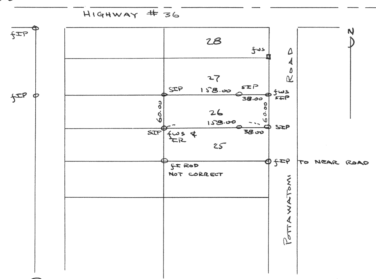
Plat of survey of lot 26, Block 2, Harbor View Subdivision, Village of Williams Bay, Section 6, T1N R17E, Walworth County, Wis. Aug. 20, 1951 Lloyd L. Jensen JCB County Surveyor
