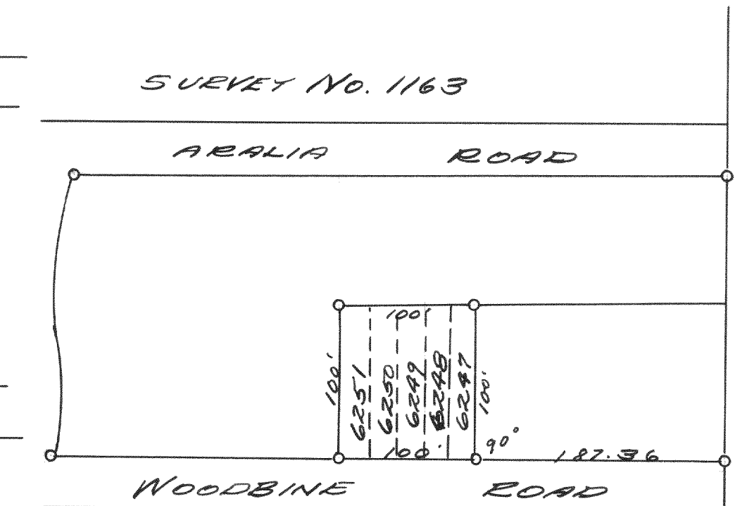
PLAT OF SURVEY OF LOTS 6247 TO 6251 OF SECTION 4 OF FELL LAKE SUBDIVISION
