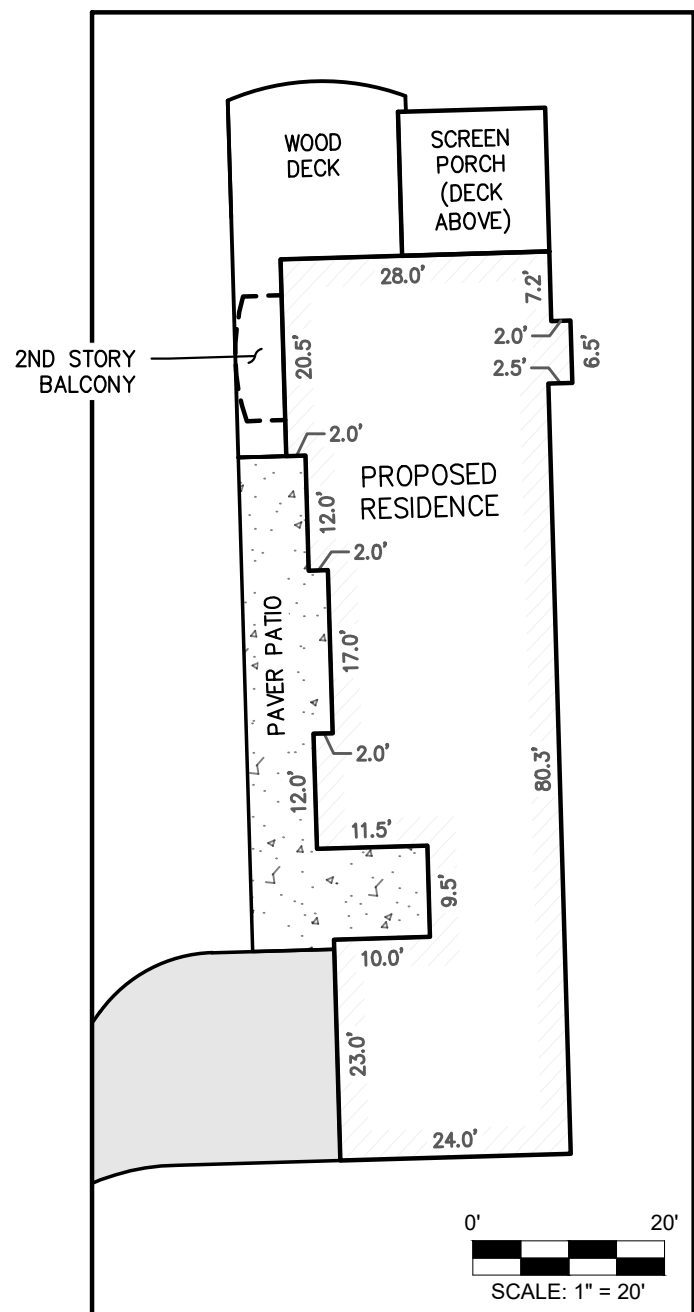
BUILDING DETAIL
